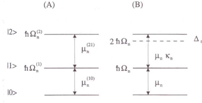
FIG. 1: (A) Basic parameters (energies and transition dipole moments) of a three level molecule, (B) anharmonic oscillator parameters representing the same system
